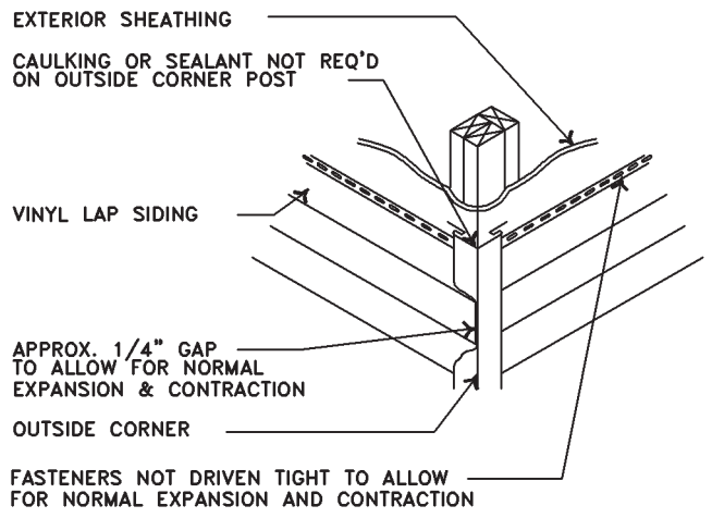
CORNER APPLICATION
