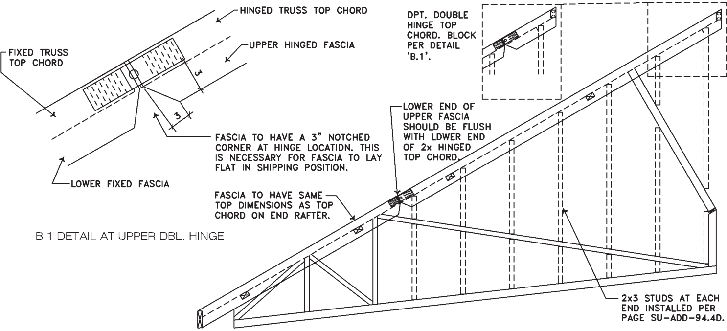
HINGED TRUSS IN RAISED SETUP POSITION
