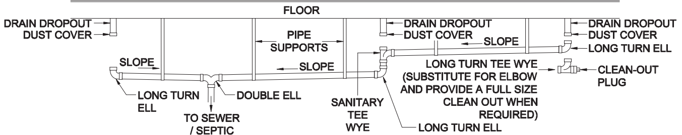
Figure 48. DWV system
