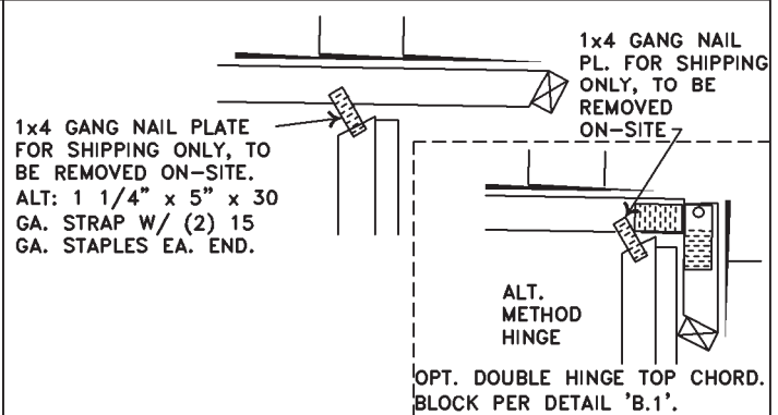
GANG NAIL/LATERAL BRACING DETAIL
