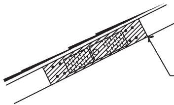
B.1 DETAIL AT UPPER DBL. HINGE
