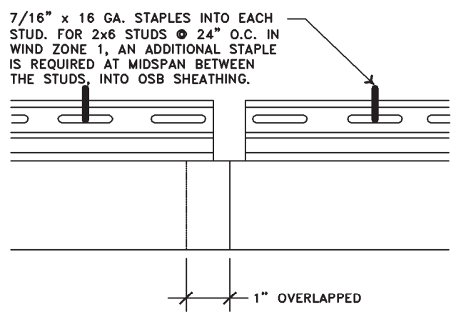
FASTENER LOCATION
