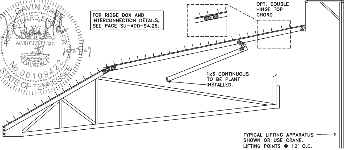
LIFTING OF HINGED TRUSS
