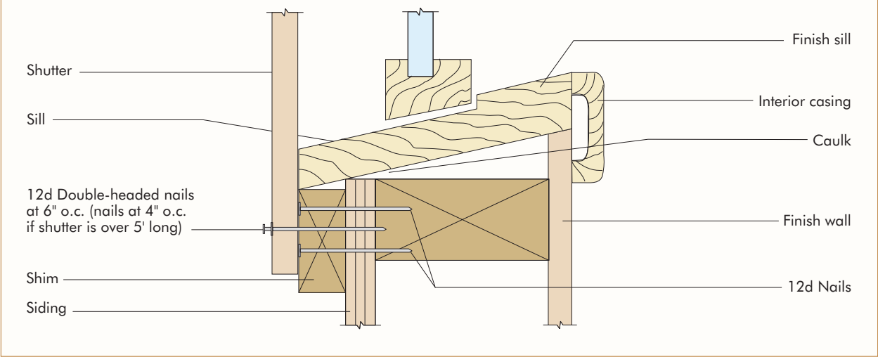
FIGURE 1C
