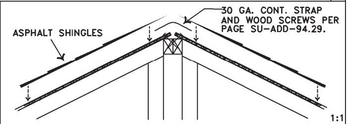
RAIL AND ROOF CONNECTION AT MATE WALL
