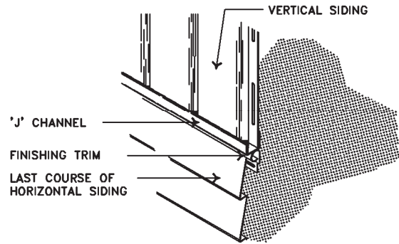
D 'J' CHANNEL
